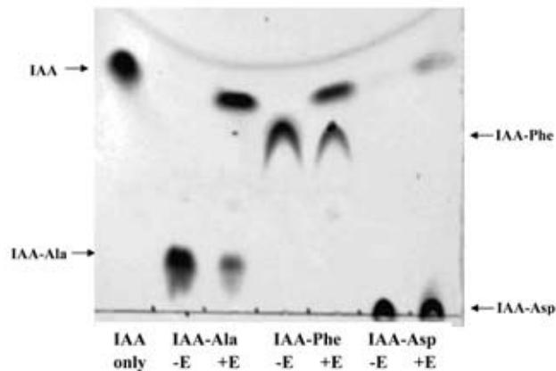
Figure 7. Enzyme activity assay of purified IAALAH with IAA-Ala, IAA-Phe, and IAA-Asp as substrates. Lane 1 was IAA standard alone, and lanes 2, 4, and 6 were reaction mixes with substrates of IAA, IAA-Ala, IAA-Phe, and IAA-Asp, respectively, but without IAALAH.
