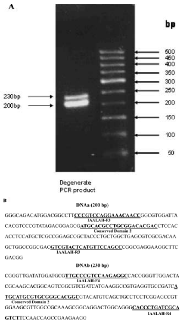
Figure 2. The degenerate PCR results analyzed on a 2% TAE agarose gel electrophoresis (A) and the DNA sequencing results of the PCR products (B). Two PCR products at 200 bp (DNAa) and 230 bp (DNAb) were identified and sequenced, respectively. The specific primer pairs of IAALA-F3/IAALA-R3 and IAALA-F4/IAALA-R4 were designed and generated for further real time PCR and colony screening based on DNAa and DNAb sequences.
