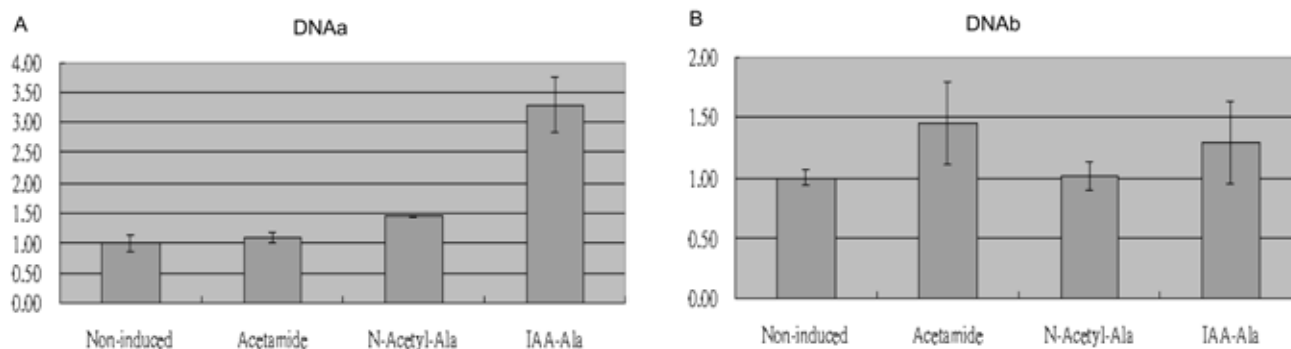
Figure 3. Expression of genes containing DNAa (A) and DNAb (B) under various induction conditions based on real time PCR analysis with IAALA-F3/IAALA-R3 for detection of DNAa and IAALA-F4/IAALA-R4 for DNAb, respectively.
