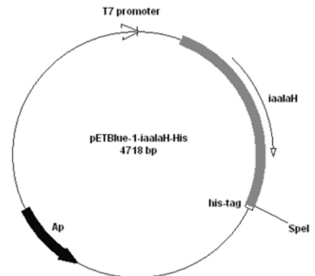
Figure 6. The pETBlue-1- iaalaH -His construct based on pETBlue-1 expression vector with iaalaH and His-tag sequences for overexpression in E. coli KRX under T7 promoter control.
