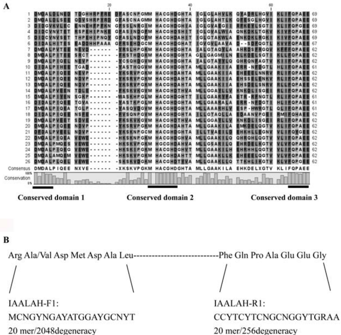
Figure 1. Partial alignment of 26 selected IAA-Asp hydrolase homologs (A) and strategy for generation of universal degenerate PCR primers for IAA amidohydrolase genes based on the conserved domains 1 and 3 (B). The protein assignments, organism names and accession numbers for the 26 protein sequences are listed as follow: 1, IAASPH (IAA-Asp hydrolase) from E. agglomerans (AF006687); 2, a putative amidohydrolase from E. coli (AE000231); 3, a probable amino acid amidohydrolase from Clostridium perfringens (AP3189); 4, a putative hydrolase from Haemophilus influenzae (U32740); 5, an unknown protein from Pasteurella multocida (AE006168); 6, a hypothetical protein from Halobacterium sp. (AE004999); 7, a theoretical N -acyl-L-amino acid amidohydrolase from Synechocystis sp. (D90917); 8, a theoretical N -acyl-L-amino acid amidohydrolase from Fusobacterium nucleatum (AE010570); 9, a theoretical N -acyl-L-amino acid amidohydrolase from Nostoc sp. (AP003598); 10, a putative hippurate hydrolase from Agrobacterium tumefaciens (AE009220); 11, an IAA-amino acid hydrolase homolog from Pyrococcus furiosus (AE010182); 12, a hypothetical amino acid amidohydrolase from Pyrococcus horikoshii (AP000003); 13, an amino acid hydrolase from Pyrococcus abyssi (AJ248287); 14, a thermostable carboxypeptidase from Sulfolobus solfataricus (AE006750); 15, a putative amino acid amidohydrolase from E. coli (AP002567); 16, a putative hippurate hydrolase from Sinorhizobium meliloti (AL591784); 17, a probable hydrolase from Pseudomonas aeruginosa (AE004718); 18, a putative N -acyl-L-amino acid amidohydrolase from Deinococcus radiodurans (AE001894); 19, a thermostable carboxypeptidase from S. solfataricus (AE006803); 20, a hypothetical amidohydrolase from P. horikoshii (AP000004); 21, an N -acyl-L-amino acid amidohydrolase from Staphylococcus aureus (AP003359); 22, ILL1 from A. thaliana (U23795); 23, a putative IAA-Ala hydrolase from Oryza sativa (AP003924); 24, ILL2 from A. thaliana (U23796); 25, an IAA-amino acid hydrolase from A. thaliana (AF081067); 26, an IAA-amino acid hydrolase from A. thaliana (U23794).
